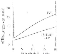
Attenuation of 24-gauge twisted pair cables with 6 to 7 mils of insulation.
